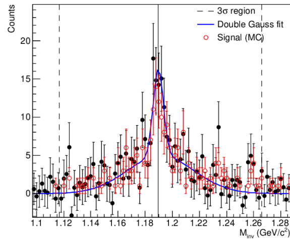
Signal [1.90-2.30] GeV/c
