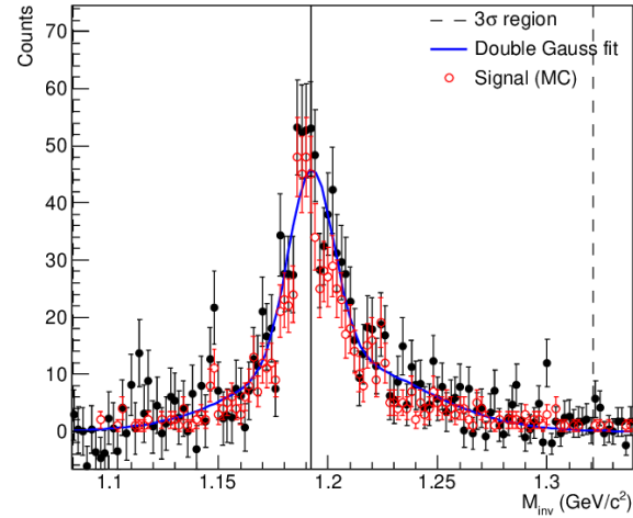
Signal [2.30-2.80] GeV/c
