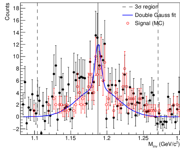
Signal [2.30-2.80] GeV/c
