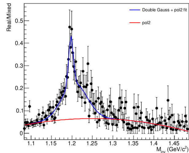
R/M Ratio [1.50-1.90] GeV/c
