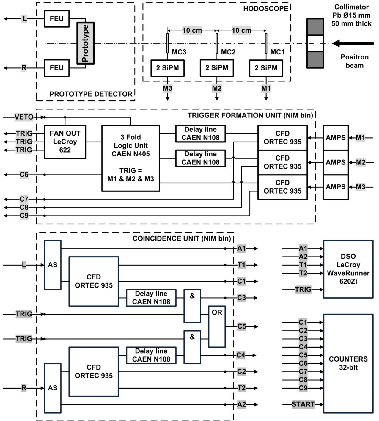
Fig. 2. Measurement setup and scheme of the data acquisition: FEU – front-end unit. L and R – analog signals from «left» and «right» ends of prototype detector respectively; A1÷A2 – signals for amplitude analysis; T1÷T2 – signals for temporal analysis; C1÷C9 – counting signals. VETO and START – logical external control signals from remote workstation; DSO – remotely operated digital oscilloscope LeCroy WaveRunner 620Zi. MC1÷MC3 - hodoscope of three 3x15x15 mm 3 SC-301 polystyrene scintillation counters wrapped with MYLAR reflection material. The triple coincidence signal from hodoscope's counters (signals M1÷M3) forms the trigger signal TRIG with duration of 20 ns. The measured time resolution of the hodoscope is 104 \pm 2 ps. AS – analog splitter; CFD – constant fraction discriminator type ORTEC 935; &, OR – AND, OR double coincidence logic type LeCroy 622; AMPS - preamplifier-shaper with pole-zero cancellation circuit.
