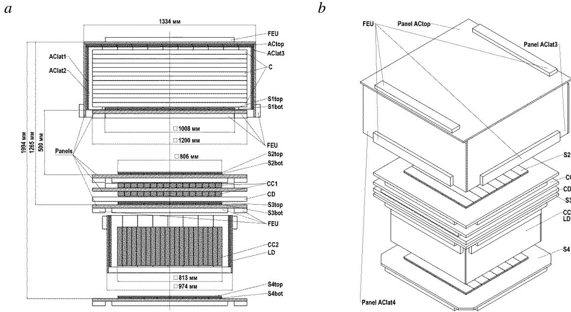
Fig. 1. The physical scheme of the GAMMA-400 gamma-ray telescope.
