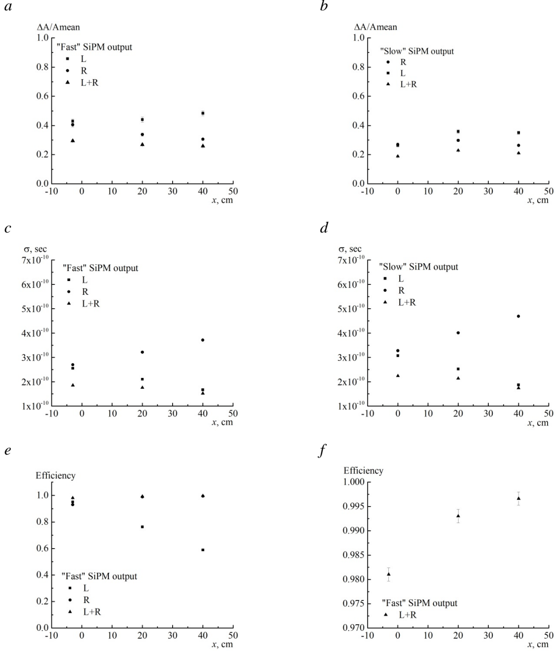
Fig. 3. The amplitude resolution (a, b), time resolution (c, d) and detection efficiency (e, f) of the prototype detector as a function of the beam impact position x relative to the detector center for «fast» (a, c, e, f) and «slow» (b, d) SiPM output, respectively. Fig. 2f shows the overall L+R efficiency from Fig. 2e on an enlarged scale. \Delta A – FWHM of the amplitude distribution, A_{\text{mean}} – mean value of the amplitude. The designators L and R correspond to the «left» and «right» ends of the scintillator strip, respectively. L+R – combined resolution \sigma_{\text{LR}} at both ends obtained as 1/\sigma_{\text{LR}}^2 = 1/\sigma_{\text{L}}^2 + 1/\sigma_{\text{R}}^2 for Figs. 2a-2d and logical sum (by OR) of signals from both strip ends for Figs. 2e-2f. Error bars are less than some points on the plots.
