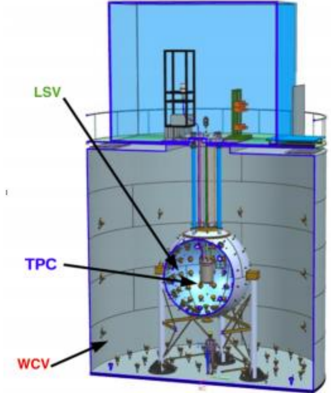
DarkSide-50
