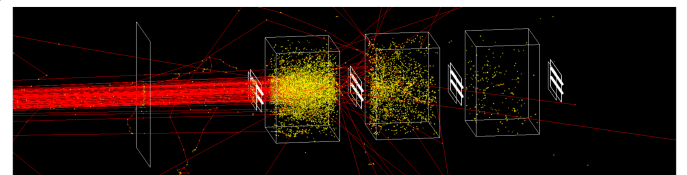
Fig.5 GEANT4 simulation of electron beam with 200 MeV energy. Red lines are electrons, green lines of photons are deleted (see Table 3), the lead absorbers are 3 cm thick.
