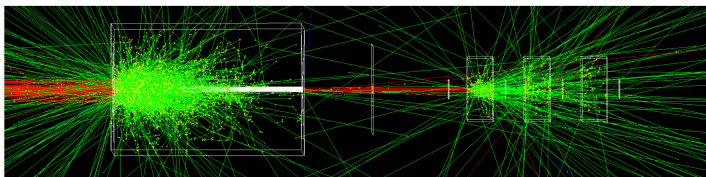
Fig.4 GEANT4 simulation of electron beam with 150 MeV energy. Red lines are electrons, green lines are photons.
