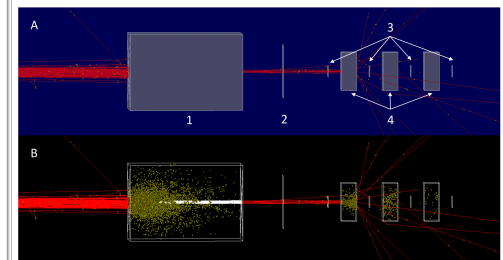
Fig.2 GEANT4 simulation experimental setup. A - the general scheme of the experimental setup, B - the same, with transparent volumes. Red lines are the electron tracks, yellow dots indicate the interaction points. The photon tracks were removed from the picture.
