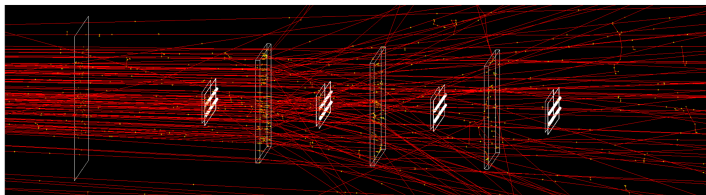
Fig.3 GEANT4 simulation of electron beam with 50 MeV energy. Red lines are electrons, lines of photons were removed.
