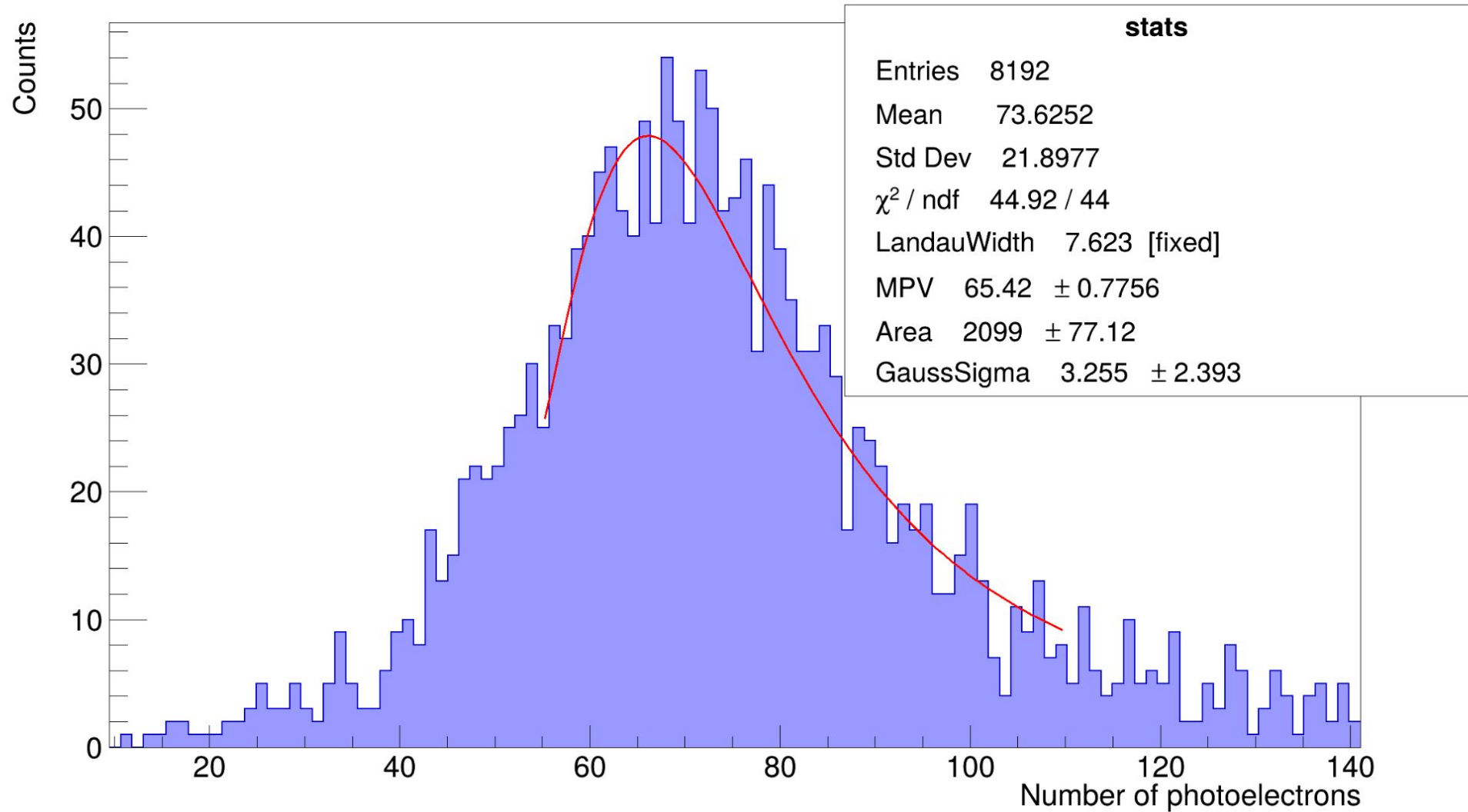
Photoelectrons spectrum (experiment)
