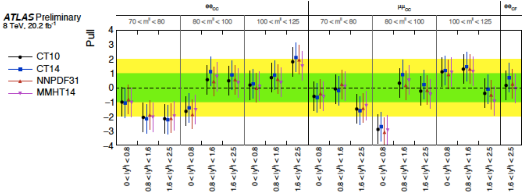
Figure 8: For 19 out of 20 measurement bins over the three analysis channels, distribution of the pulls of each measurement of \sin^2 \theta_{\text{eff}}^\ell with respect to a reference chosen to be the most sensitive measurement, namely that from the ee_{CF} channel in the measurement bin 2.5 < |y^{\ell\ell}| < 3.6 . The results are shown separately for the four different PDF sets considered in this note.
